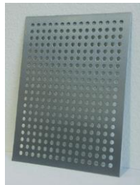
Perforation diameter 8 mm, holes in a grid spaced at 15 x 15 mm
